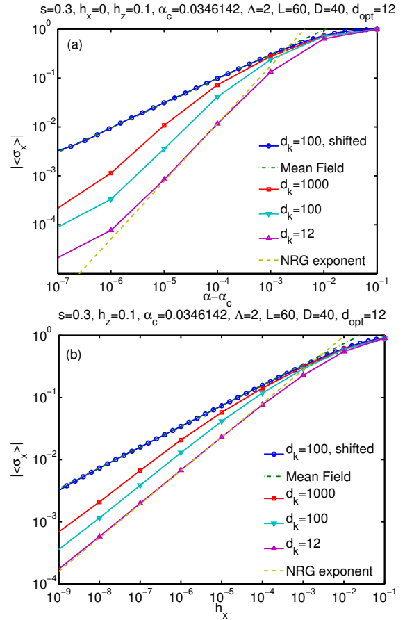
FIG. S6: The effect of Hilbert space truncation on the calculation of the SBM1 critical exponents \beta in (a) and \delta in (b). The calculation labeled “ d_k = 100 , shifted” was performed using the OBB method with explicit shifts, without setting any maximum value for the size of the shifts, i.e. without restricting d_k^{\text{eff}} . Dashed straight lines correspond to power laws with exponents \beta_{\text{NRG}} = 1.18 and \delta_{\text{NRG}} = 1.85 obtained by NRG 13 . \delta_{\text{NRG}} agrees with the hyperscaling exponent \delta = (1+s)/(1-s) that applies for s > 1/2 , see Sec. IV C below. 16
