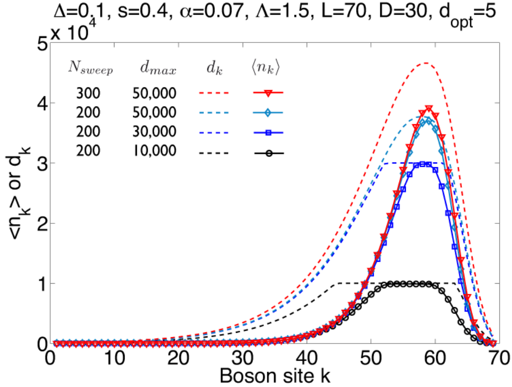
Figure 4.7: The boson occupation (solid lines with symbols) and dynamically determined d_k (dashed lines) of the boson sites. d_{max} is the upper limit of d_k set by hand to show the effect of limiting d_k . N_{sweep} is the number of VMPS sweeps. The results is obtained in the localized regime of SBM1.
