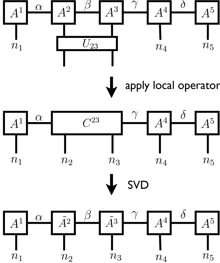
Figure 2.10: Schematic diagram of applying a local operator U^{23} on a MPS. First contract the local indices on site 2 and 3 with the indices of U^{23} . This will result a big tensor C^{23} . Then a singular value decomposition is performed to restore the original MPS structure. [See Eq. (2.43)]
