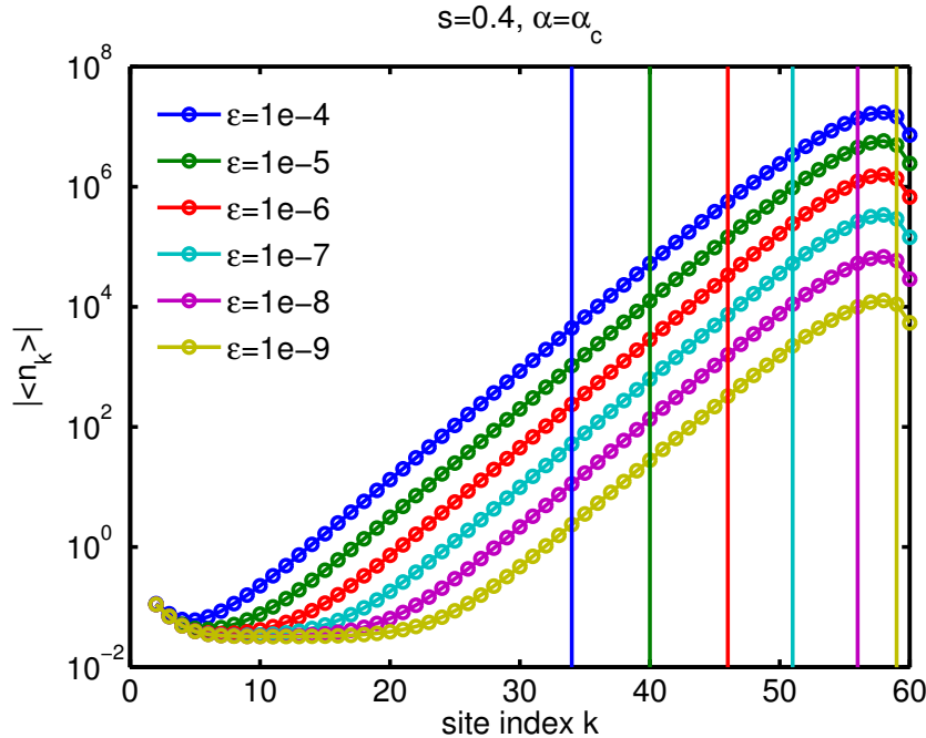
Figure 4.2: Same as Fig. 4.1 except for several different \epsilon at \alpha = \alpha_c , which is calculated at \epsilon = 0 .
