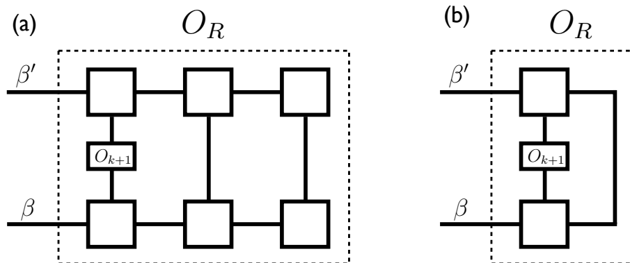
Figure 2.13: Transforming the local operator into the right block basis. The whole structure inside the dashed line is O_R . Because all matrices shown in this plot are assumed to be right-orthonormalized (a) can be reduced to (b).
