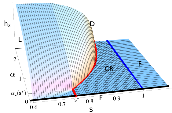
FIG. S10: Schematic sketch of the SBM2 phase diagram as function of s , \alpha and h_z . The localized phase (L) lies below the curved surface representing the critical field h_z^c(s, \alpha) , the delocalized phase (D) above and to its right. (The curved surface was not calculated, but is an artist’s impression.) The cross-hatched area in the h_z = 0 plane represents the critical phase (CR). Its phase boundary with the localized phase (L) is marked by the thick red line in the h_z = 0 plane (corresponding to the red line in main text, Fig. 3a), consisting of a straight line between the points (s^*, 0) and (s^*, \alpha_c(s^*)) , and a curved portion representing the line \alpha_c(s) , for s^* < s < 1 . The thick blue line at s = 1 is the CR-F phase boundary to the free phase (F). The thick black line at \alpha = h_z = 0 likewise represents a free spin (F).
