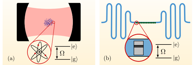
FIG. 1 (color online). Cavity QED system with N atoms (a) and circuit QED system with N Cooper-pair boxes as artificial atoms (b).
