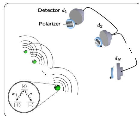
FIG. 1 (color online). Proposed experimental arrangement. N excited emitters are aligned in a row, each of them defining a three-level \Lambda system. A long-lived entangled state is obtained in the N emitter qubits after detecting the N spontaneously emitted photons with N detectors equipped with polarizers. The final N -qubit state is tuned and determined by the polarizer orientations.
