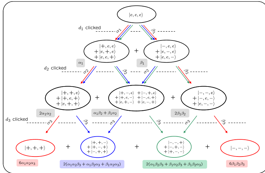
FIG. 2 (color online). Pyramid of entanglement paths for the case of 3 emitters initialized in the excited state |e, e, e\rangle . The figure illustrates the intermediate states, horizontally displayed, during three successive photodetection events realized by three detectors d_1 , d_2 , and d_3 , equipped with general elliptical polarizers oriented along \boldsymbol{\epsilon}_1 , \boldsymbol{\epsilon}_2 , and \boldsymbol{\epsilon}_3 ( \boldsymbol{\epsilon}_i \equiv \alpha_i\boldsymbol{\sigma}_+ + \beta_i\boldsymbol{\sigma}_- ), respectively. After each detection, the unnormalized global state of the system is the sum of all states in the circles weighed by the tagged prefactors. Left-down arrows denote \boldsymbol{\sigma}_+ transitions, and right-down arrows represent \boldsymbol{\sigma}_- ones. The final state components are shown inside colored frames and the colored arrows represent the quantum paths leading to these different components. Only the red (gray) circle states are obtained via a single quantum path, while the blue (dark gray) and green (light gray) ones are the result of three different interfering quantum paths.
