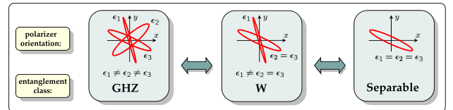
FIG. 3 (color online). Operational monitoring of tripartite entanglement classes by changing the polarization configurations. If the three polarizer orientations are all different, the final state belongs to the \text{GHZ} class; if two polarizer orientations are different, the final state belongs to the W class; if all polarizers are identically oriented, the final state belongs to the S class.
