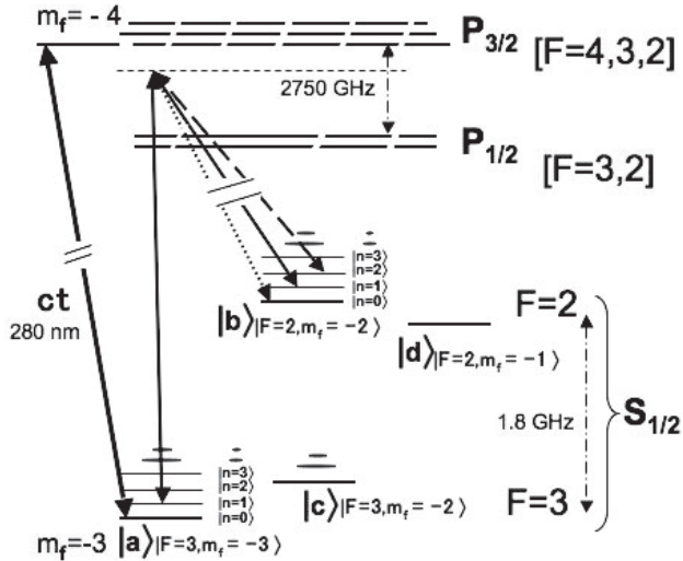
FIG. 1. Energy levels of a ^{25}\text{Mg}^+ ion confined in a trap [22,23]. Shown are the relevant types of two-photon Raman transitions between states |a, n=1\rangle and |b, n=0, 1, 2\rangle : red sideband (dotted line), carrier (solid line) and blue sideband (dashed line); see also the resonant transition for state sensitive detection. We subsumed excited levels of the P_{1/2} and P_{3/2} states.
