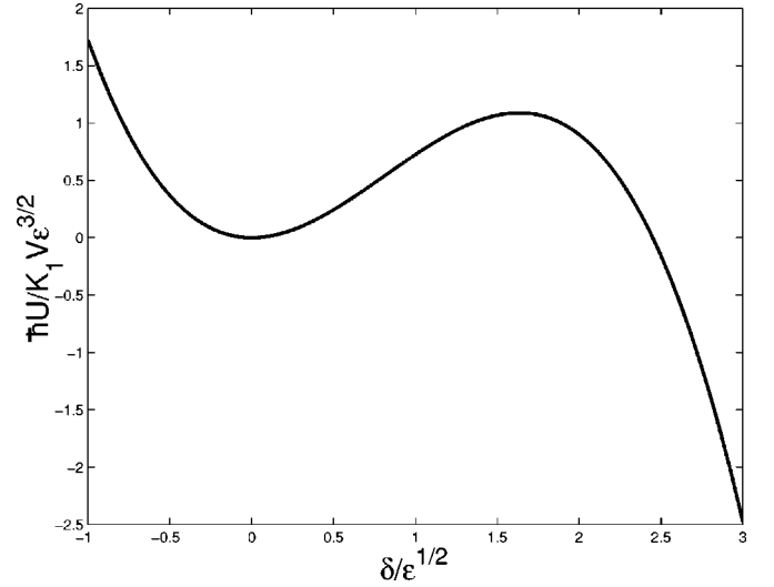
FIG. 2. The \delta (= \theta - \theta_0) dependence of the effective potential \hbar U / K_1 V \epsilon^{3/2} for \theta_H = 3\pi/4 (the phenomenon of MQT).
