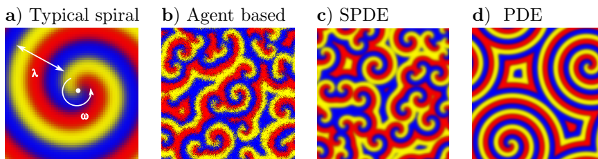
Figure 16: Spiral patterns . a) Schematic drawing of a spiral with wavelength \lambda . It rotates around the origin at a frequency \omega . b) Agent-based simulations for D < D_c , when all three species coexist, show entangled, rotating spirals. c) Stochastic partial differential equations, discussed in section 4.4, show similar patterns as agent-based simulations. d) Spiral pattern emerging from the dynamics of the deterministic diffusion reaction equation starting from a spatially inhomogeneous initial state. Parameters are \sigma = \mu = 1 and D = 1 \times 10^{-5} . Figure adapted from Ref. [73].
