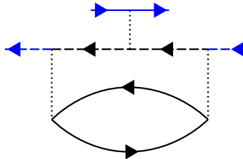
Figure 4.9.: Third order irreducible vertex diagram, contributing as V_0 g^2 L , which is subleading.
