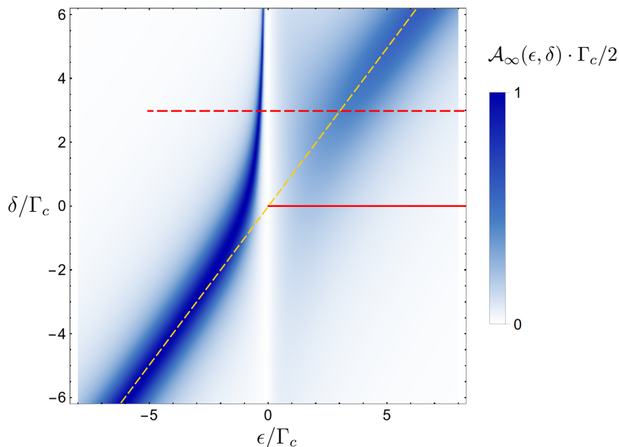
Figure 5.2.: Fermi-edge polariton spectral function for infinite hole mass. This plot was generated by inserting the infinite hole mass photon self-energy of (3.20), (3.21) into the spectral function of (5.3). The full/dashed red lines indicate the spectral ranges shown in detail in Fig. 5.3/Fig 5.5. The dashed yellow line shows the bare photon mode. Used parameters: g_{\text{fp}} = 0.33\Gamma_c , \xi = 4\Gamma_c , g = 0.5 .
