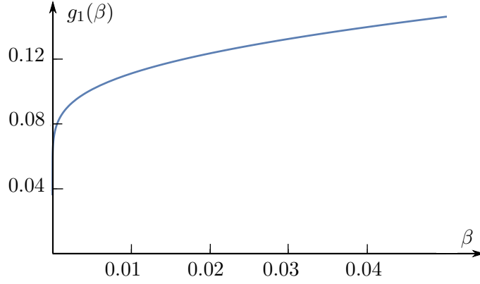
Figure 3.9.: Plot of g_1(\beta) for very small values of \beta .
