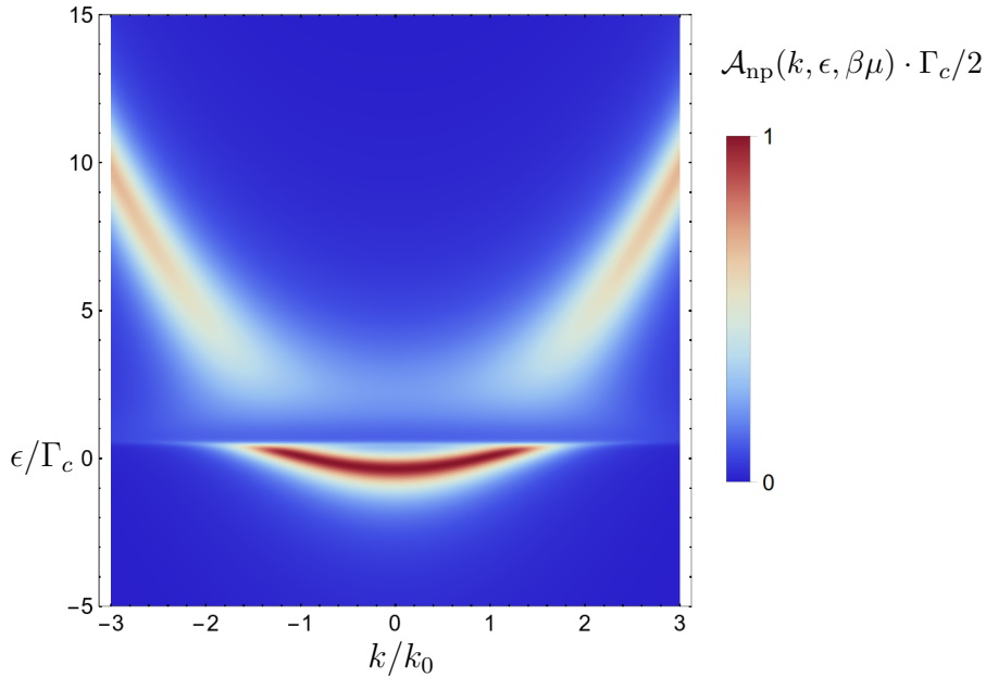
Figure 5.12.: Fermi-edge polariton dispersion spectrum \mathcal{A}_{\text{np}}(k, \epsilon, \beta\mu) for finite masses, and in the non-perturbative regime.
