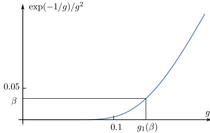
Figure 3.8.: Evaluation of the separating value g_1(\beta) .
